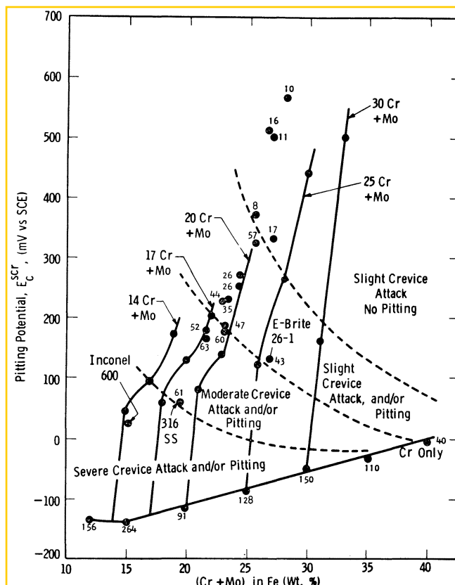
FIGURE 22 – Relationship between the critical pitting potentials ( E_c^{scr} ) measured in deaerated synthetic seawater at 90 C, pH = 7.2 \pm 0.2 of Fe-Cr-Mo based alloys and their resistance to crevice attack after a 14 day exposure to synthetic seawater at 121 C and \sim 60 ppm oxygen. The numbers associated with individual points indicate the weight losses expressed as gms \times 10^{-2} after the 121 C exposure for samples with initial weights of \sim 1 gm.
