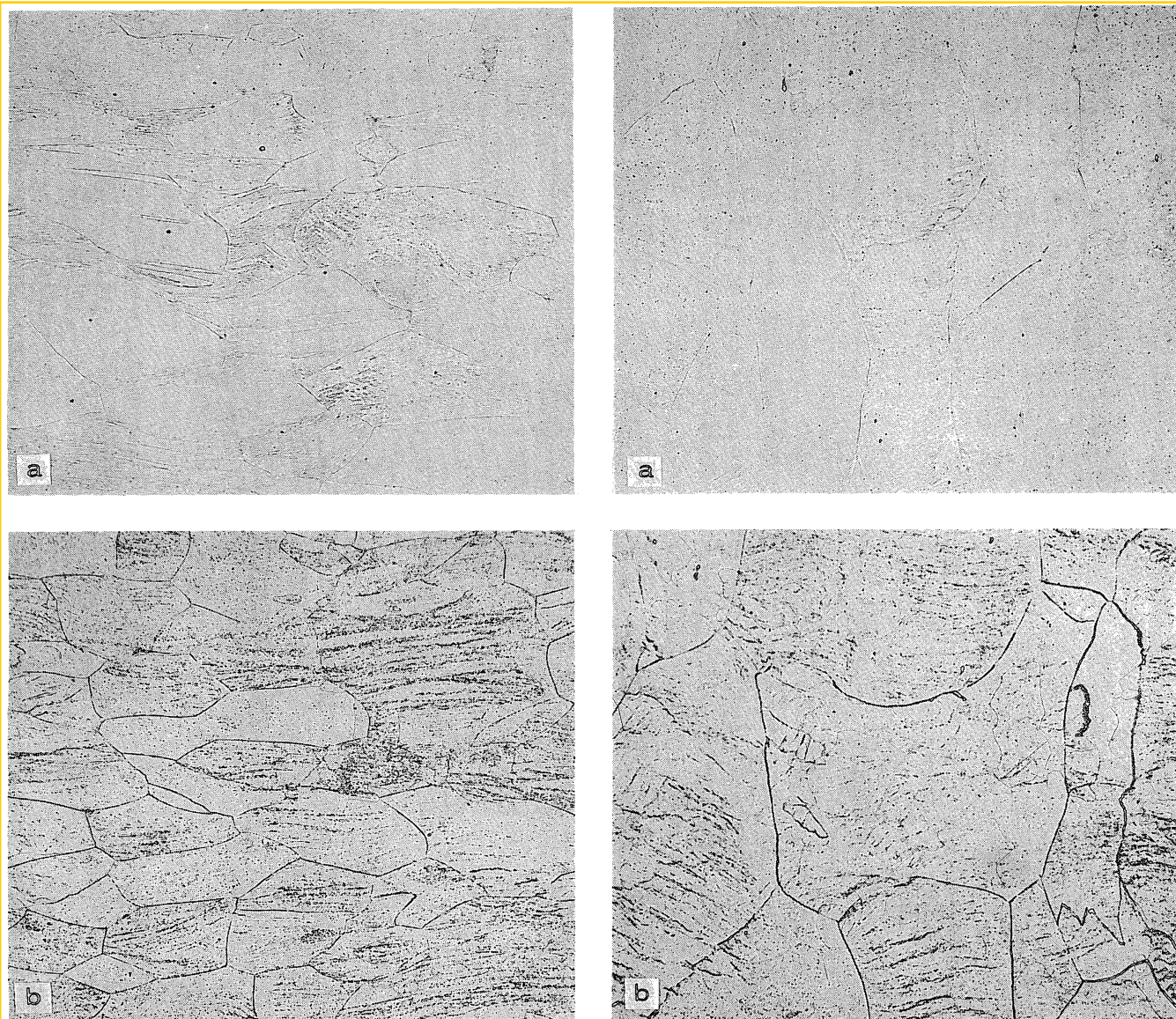
FIGURE 20 — Microstructure of E-Brite 26-1. Left column: transverse to rolling direction; right column: parallel to rolling plane. Electrolytic etch: 10% oxalic acid. (a) Alloy WE02, as cold rolled and (b) alloy WE62, as cold rolled + 788 C/1 hour. 41X
