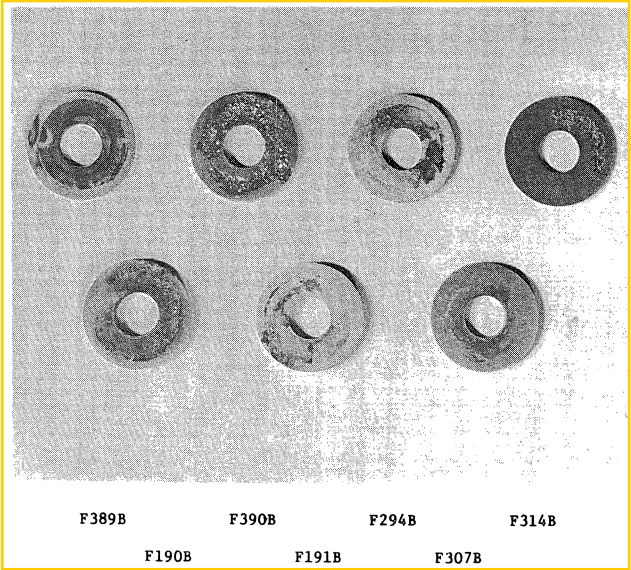
FIGURE 11 – Crevice corrosion after 342 hour exposure to synthetic seawater (pH = 7.0) at 121 C and ~ 60 ppm oxygen.
