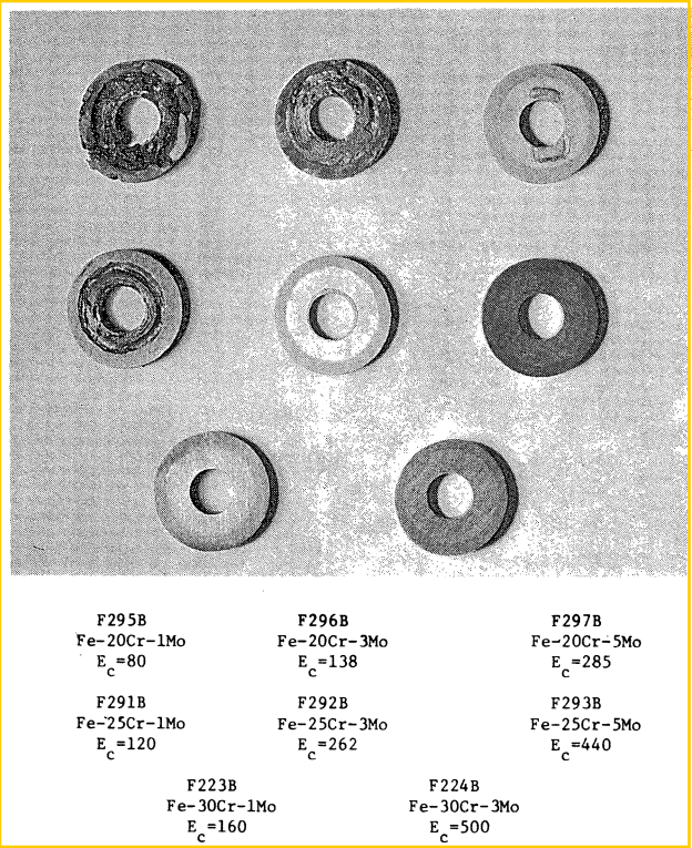
FIGURE 9 – Crevice corrosion after 6 day exposure to oxygenated 10% ferric chloride at 21 \pm 1 C. Specimen size: \frac{1}{2} inch diameter.
