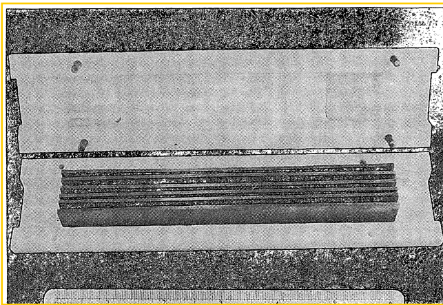
FIGURE 13 – Holder used for test coupons in desalination plant exposure tests
