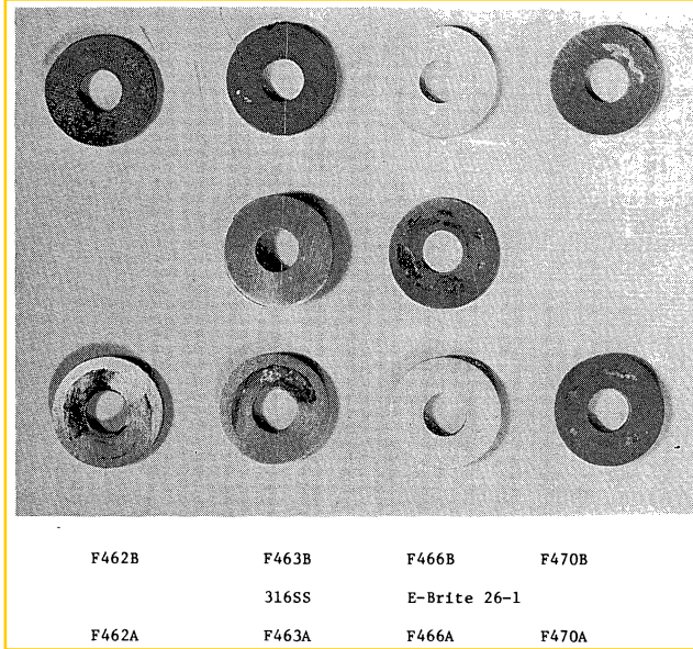
FIGURE 12 – Crevice corrosion after 342 hour exposure to synthetic seawater (pH = 7.0) at 121 C and ~ 60 ppm oxygen.
