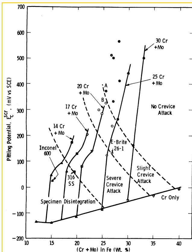
FIGURE 21 – Relationship between the critical pitting potentials ( E_c^{scr} ) measured in deaerated synthetic seawater at 90 C, pH = 7.2 \pm 0.2 of Fe-Cr-Mo based alloys and their resistance to crevice attack after a 6 day exposure in oxygenated, 10% ferric chloride at 21 \pm 1 C.
