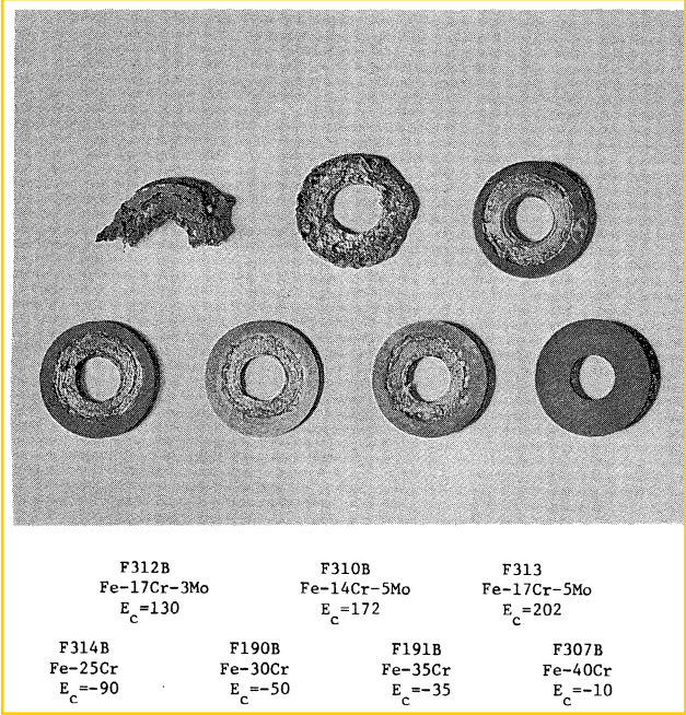
FIGURE 10 – Crevice corrosion after 6 day exposure to oxygenated 10% ferric chloride at 21 \pm 1 C. Specimen size: \frac{1}{2} inch diameter.
